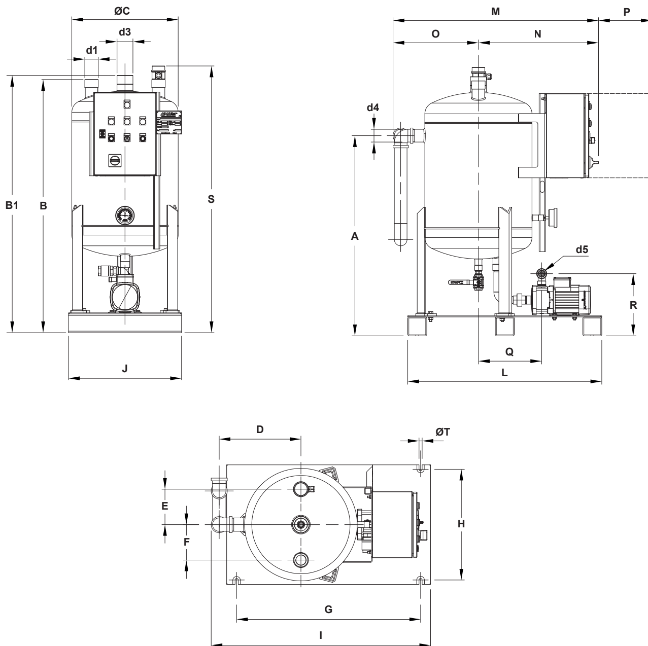
DIMENSIONS (mm) *
